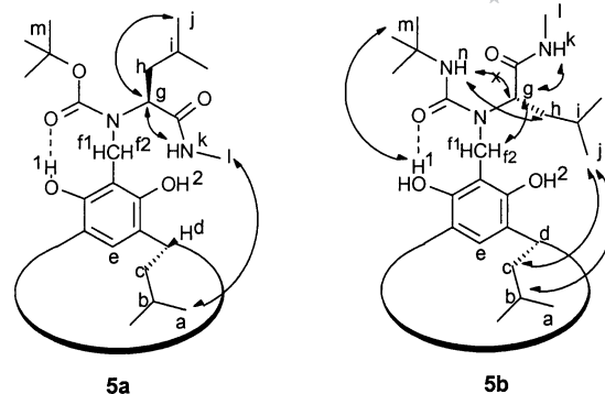
Figure 1. The most relevant ROESY contacts for 5a and 5b .
