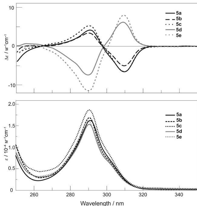
Figure 3. CD and UV spectra of 5a–e ( \text{CHCl}_3 , 303 K).
