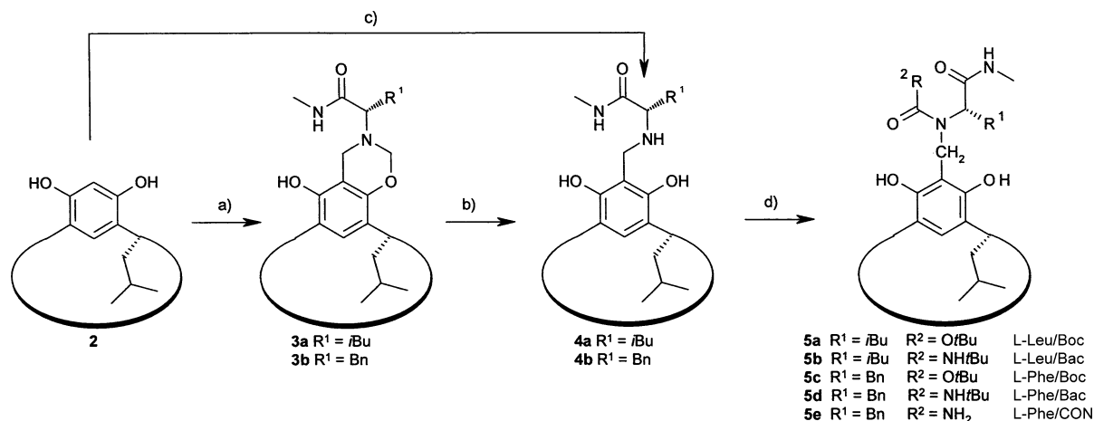
Scheme 2. Synthesis of 5a–e . Reagents and conditions: (a) aq. HCHO, L-amino acid methylamide, AcOH, MeOH; (b) ethyl nitroacetate, MeOH; (c) aq. HCHO, L-amino acid methylamide, CH 2 Cl 2 ; (d) see Experimental Section.
