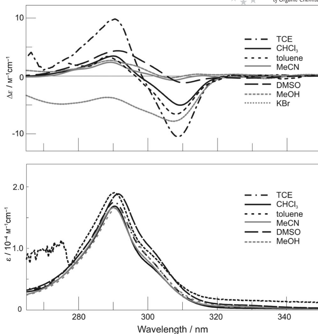
Figure 4. CD and UV spectra of 5b in various solvents and in the solid state.
