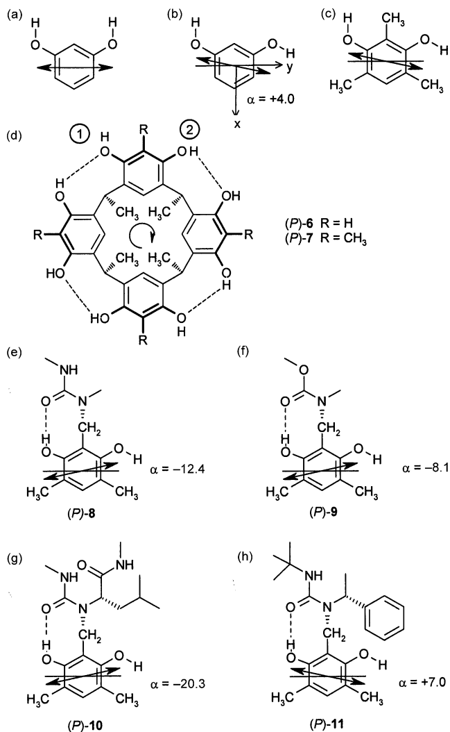
Figure 6. Model compounds for the ab initio calculations. Arrows indicate the directions of the electric dipole moments for the lowest-energy transitions as calculated by TDDFT/B3LYP/DZVP.
