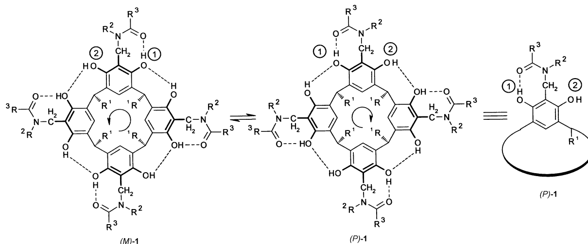
Scheme 1. Structure and stereochemical notation of conformationally inherently chiral resorcin[4]arenes.
