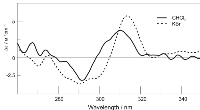
Figure 5. CD spectra of previously reported 5f [6] ( \text{CHCl}_3 solution and crystals in KBr).
