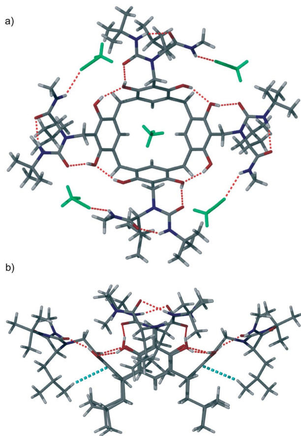
Figure 2. The crystal structure of 5b : (a) top view; lower-rim alkyl chains were removed for clarity, MeCN solvent molecules are colored in green; b) side view; solvent molecules were removed for clarity, blue dotted lines represent close CH– \pi interactions.
